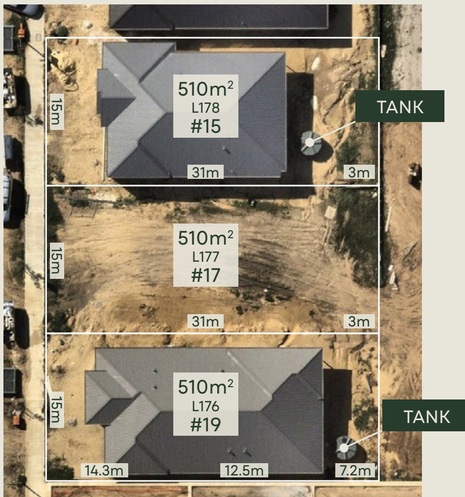
Pictured: Restricted Flood Mitigation Tank in Backyard 15 & 19 Nepean St, Margaret River
