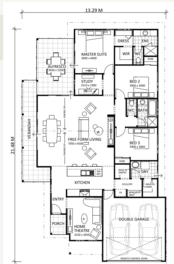
FLOOR PLAN 1:100
